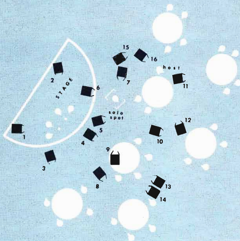
Figure 8. Low key lighting is very appropriate for cabaret or night club settings. Here, the minimum number of lights has been selected to give adequate frontal illumination to the stage, solo spot and host positions for several camera angles. The single Fresnels aimed at each of the seven tables gives a rim light effect on the faces in the audience for most camera angles. These single lights also maintain an illusion that the tables are lit by stage illumination (or possibly by the candle on each table).
